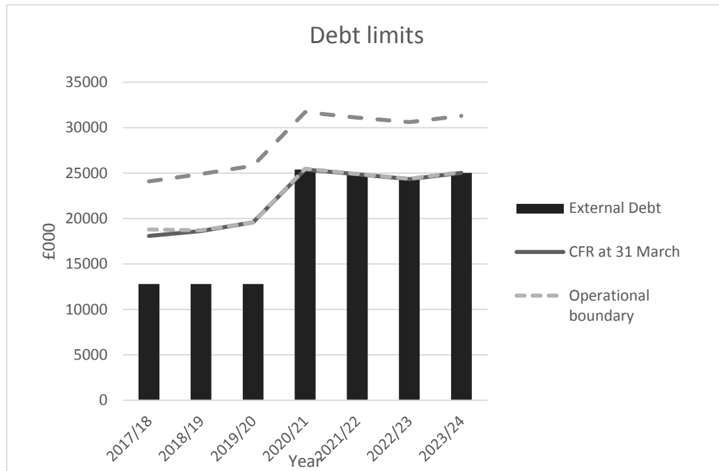
Chart 1 Borrowing v Debt limits
